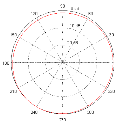
Radiation Pattern (H-Plane)
